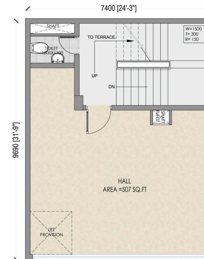
SCO FIRST FL. PLAN
